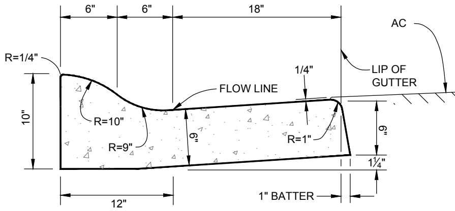
ROLLED CURB & GUTTER SECTION
