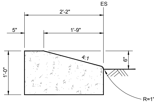
TYPE D-6 CURB
