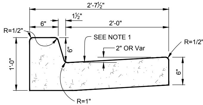
TYPE A2-6 CURB
