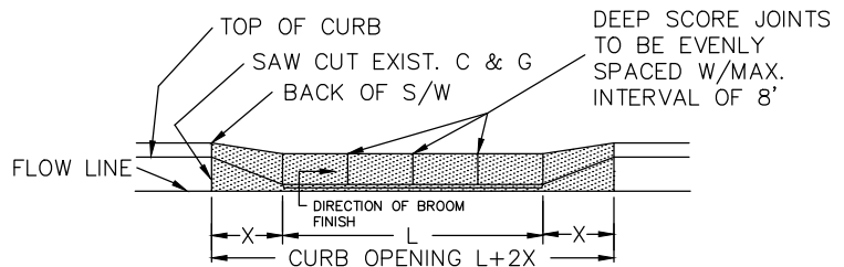
DETAIL D-5B-1
