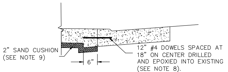
DETAIL D-5B-1
