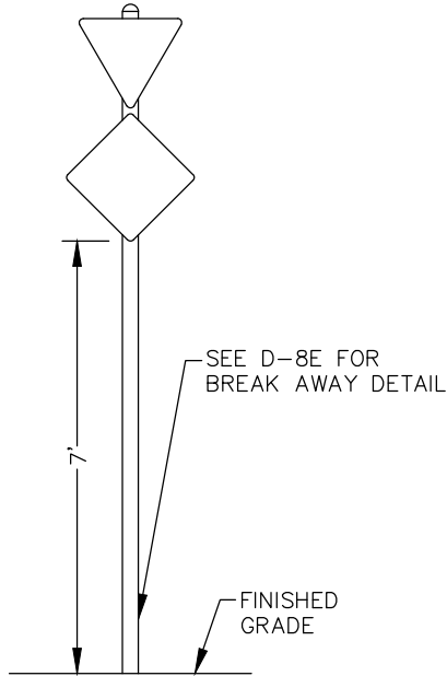
MULTIPLE SIGN DETAIL
