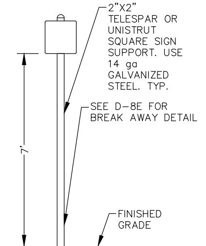
SIDEWALK OR MEDIAN DETAIL
