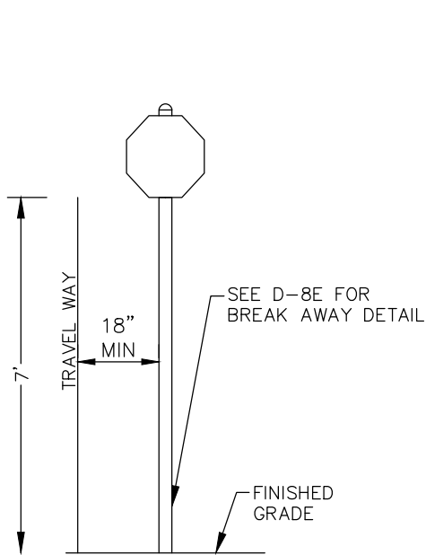
SINGLE SIGN DETAIL
