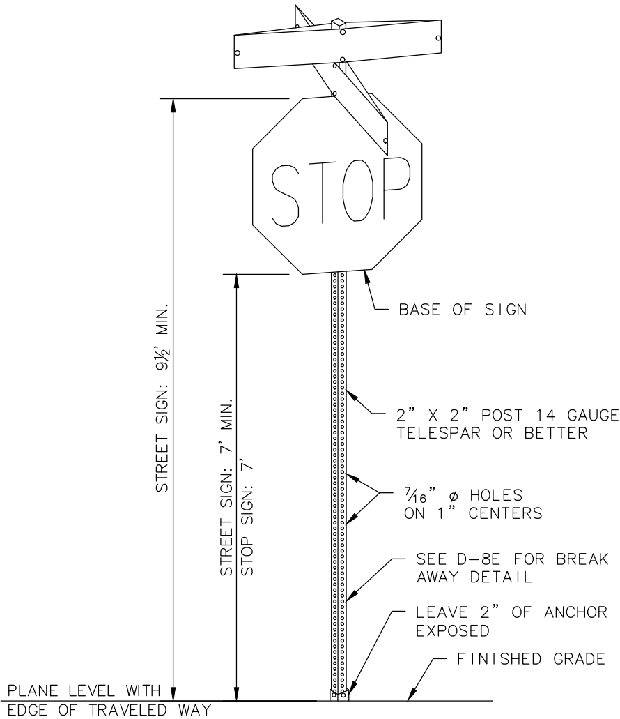
SIGN POST INSTALLATION
