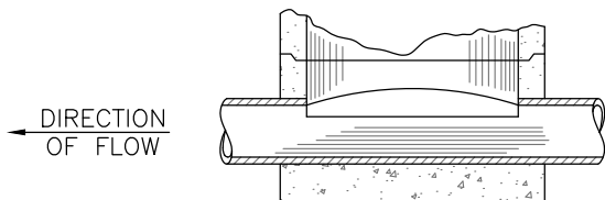
SECTION OF PIPE CONTINUOUS THROUGH MANHOLE
