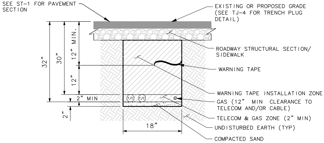
TELECOM AND GAS ONLY TRENCH
