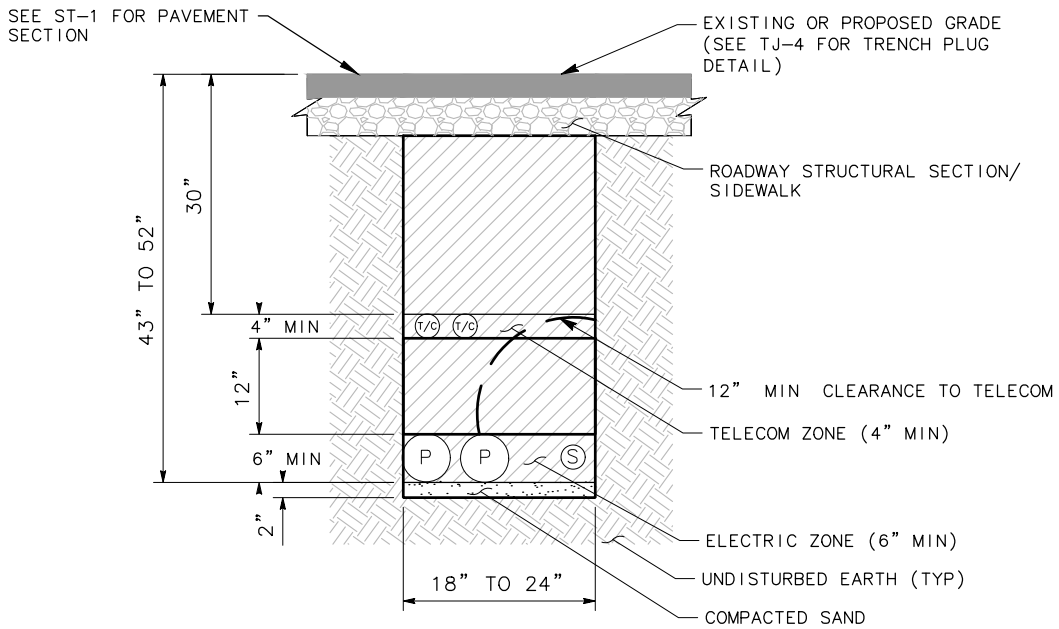
ELECTRIC & TELECOM ONLY TRENCH
